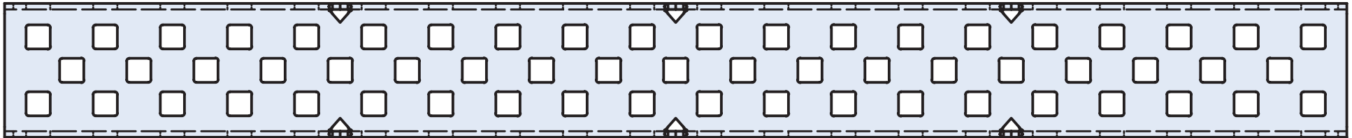
[C20] C-CHANNEL, (1X2X1) 20-HOLES LONG
